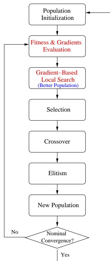
Fig. 3 Flow Chart for Gradient-Enhanced Micro-GA
